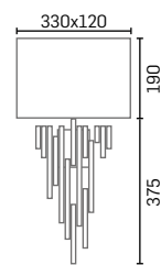
Ref.: CR17/AP 1xE27 LED
