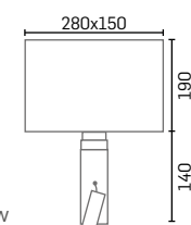
Ref.: 087/AP 1xE27 LED 1xLED Max. 1,5w
